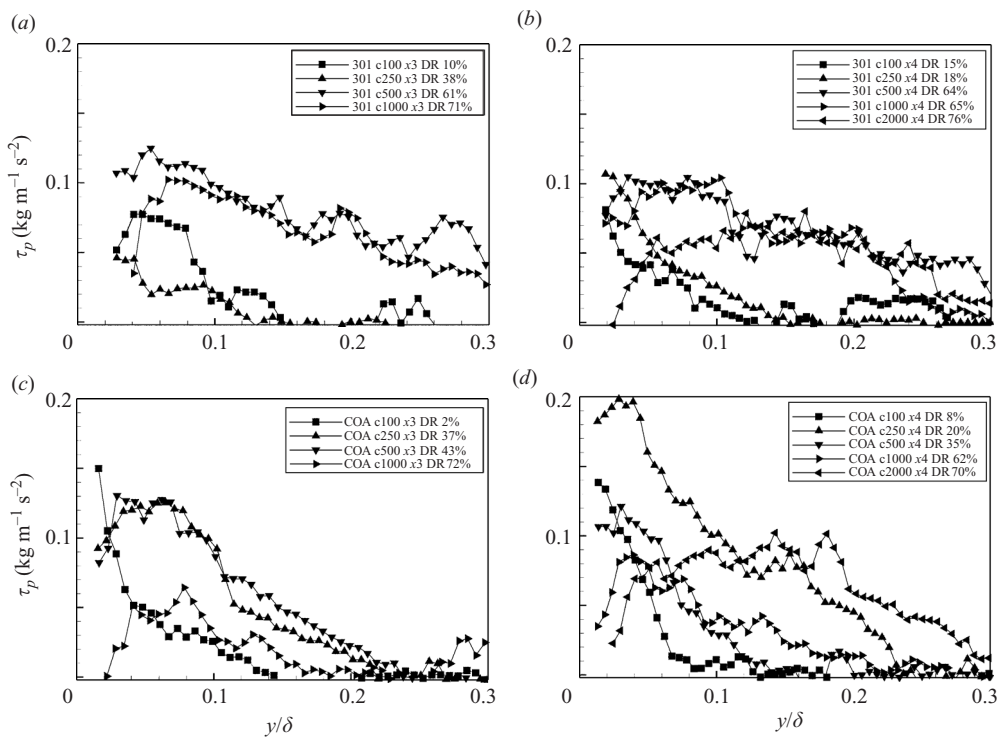
FIGURE 17 (corrected). Polymer stress profiles at fixed streamwise location for different injection concentrations.
